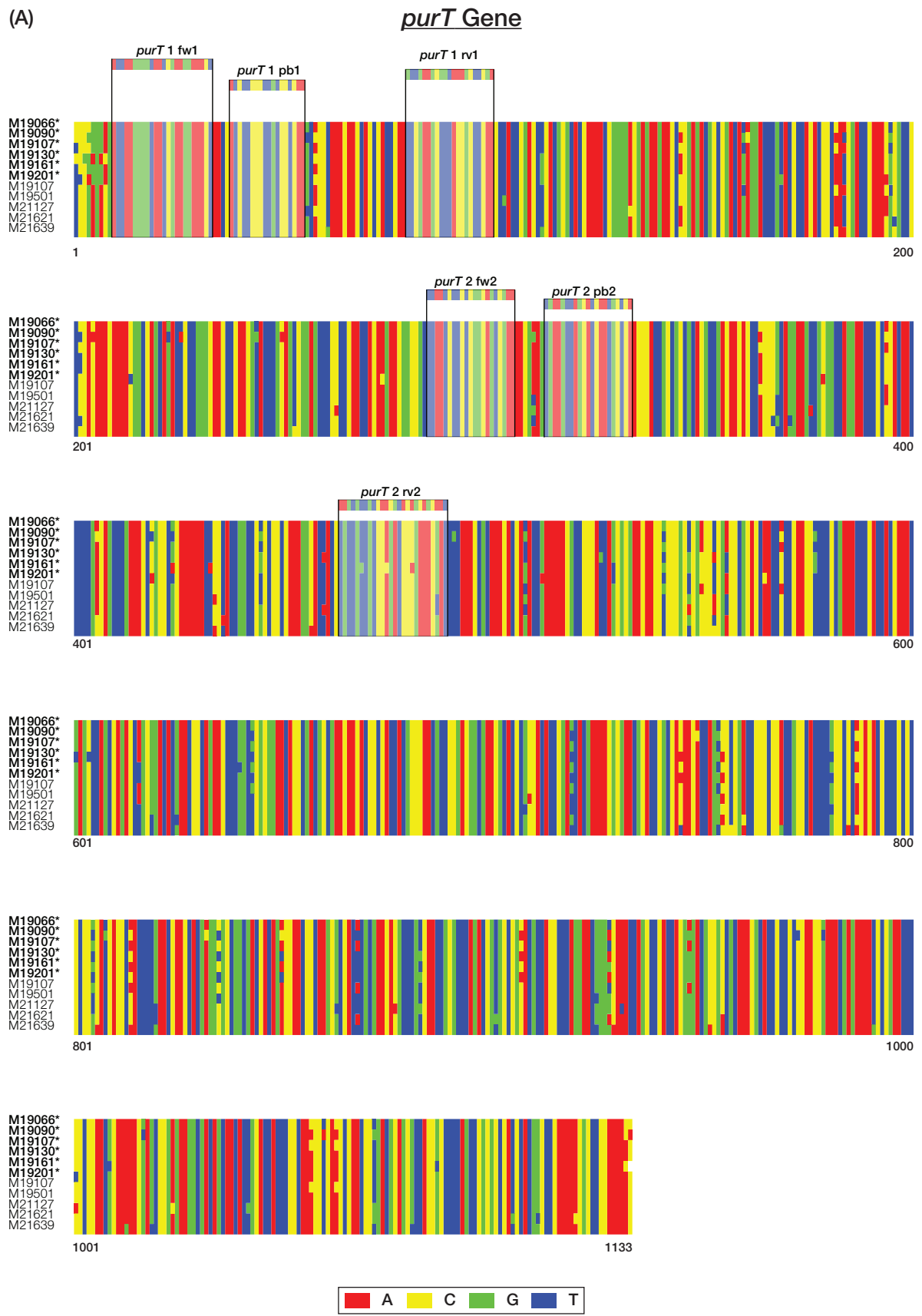
Supplementary Figure 1. Alignments of Haemophilus haemolyticus specific potential rt-PCR target genes. Alignments for (A) purT , (B) hdg and (C) sod include sequences taken from the genomes analyzed here as well as Sanger sequences ( bold with * ) of gene amplicons from additional strains. The locations of primers and probes for the purT rt-PCR assays are shown above the alignment.
